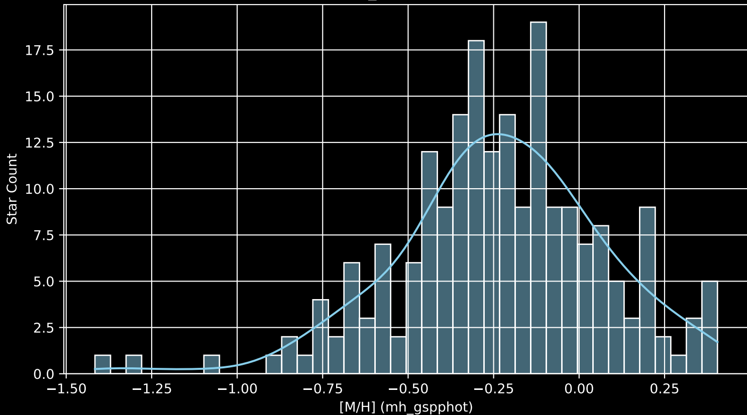
APOGEE DR17 Field: [163+78_MGA [M/H] (mh_gspphot) (n= 205)
