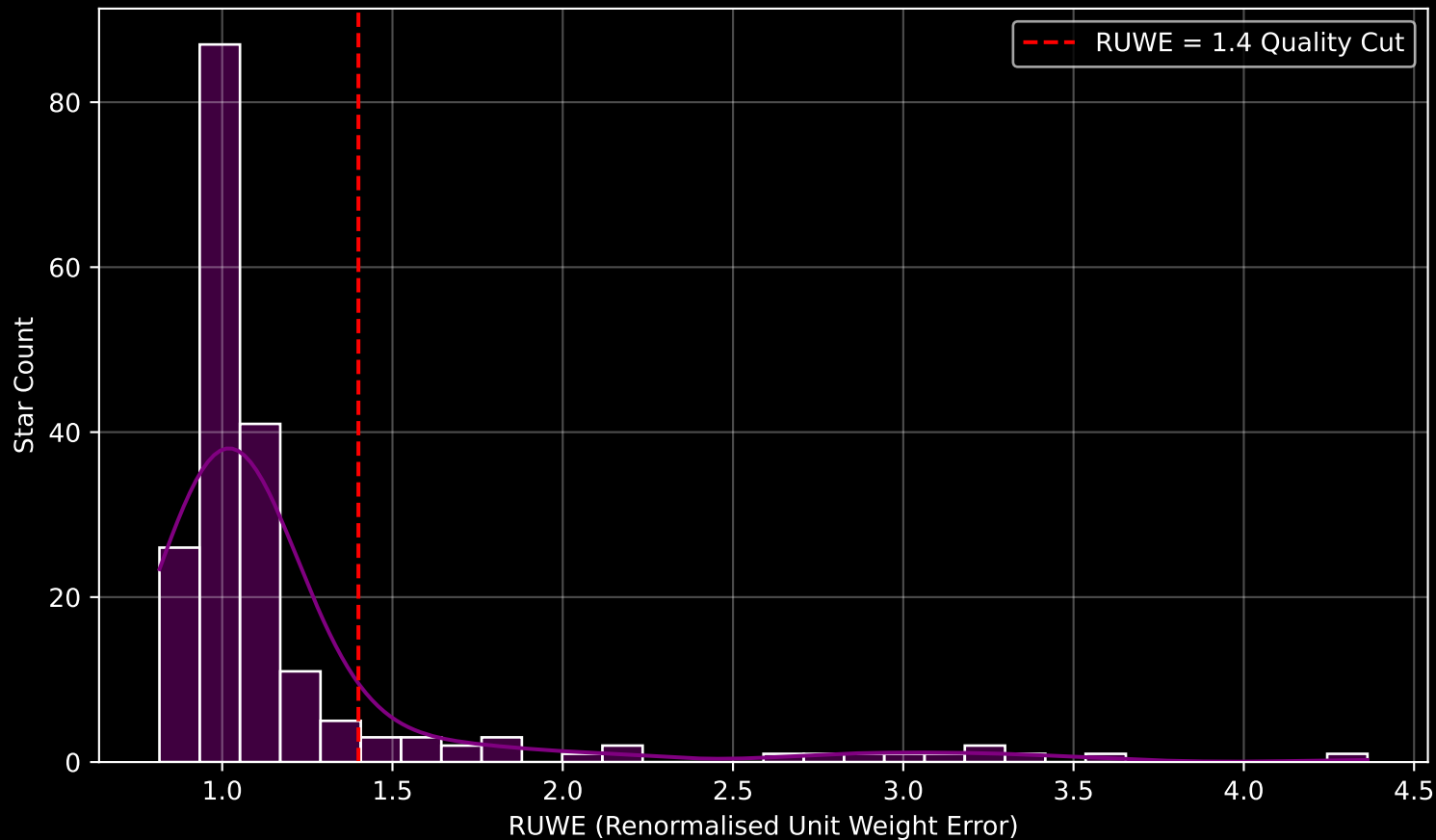
GAPOGEE DR17 Field [163+78_MGA] RUWE Distribution (n= 194)
