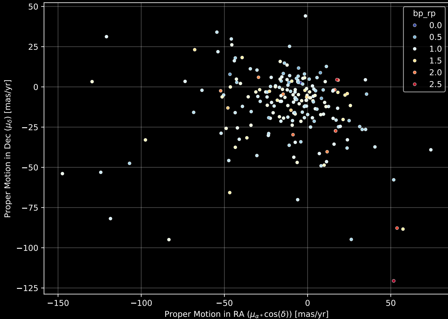
APOGEE DR17 Field: [163+78_MGA] Proper Motion Diagram (n= 207)
