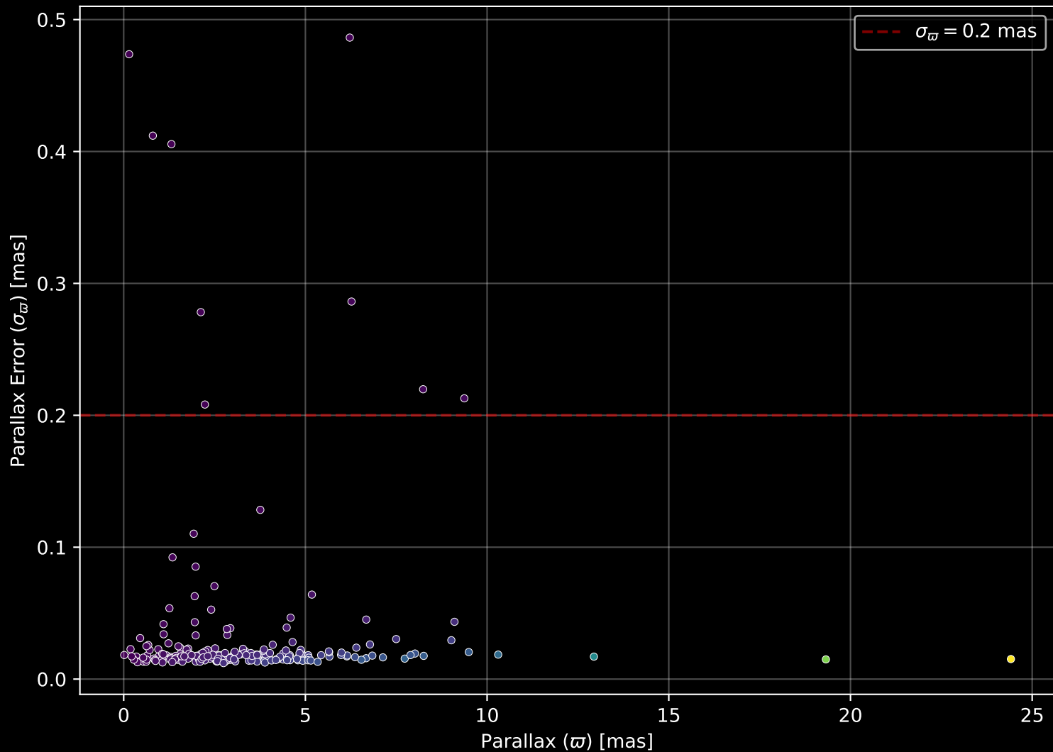
APOGEE DR17 Field: [163+78_MGA] Parallax Quality (n= 207)
