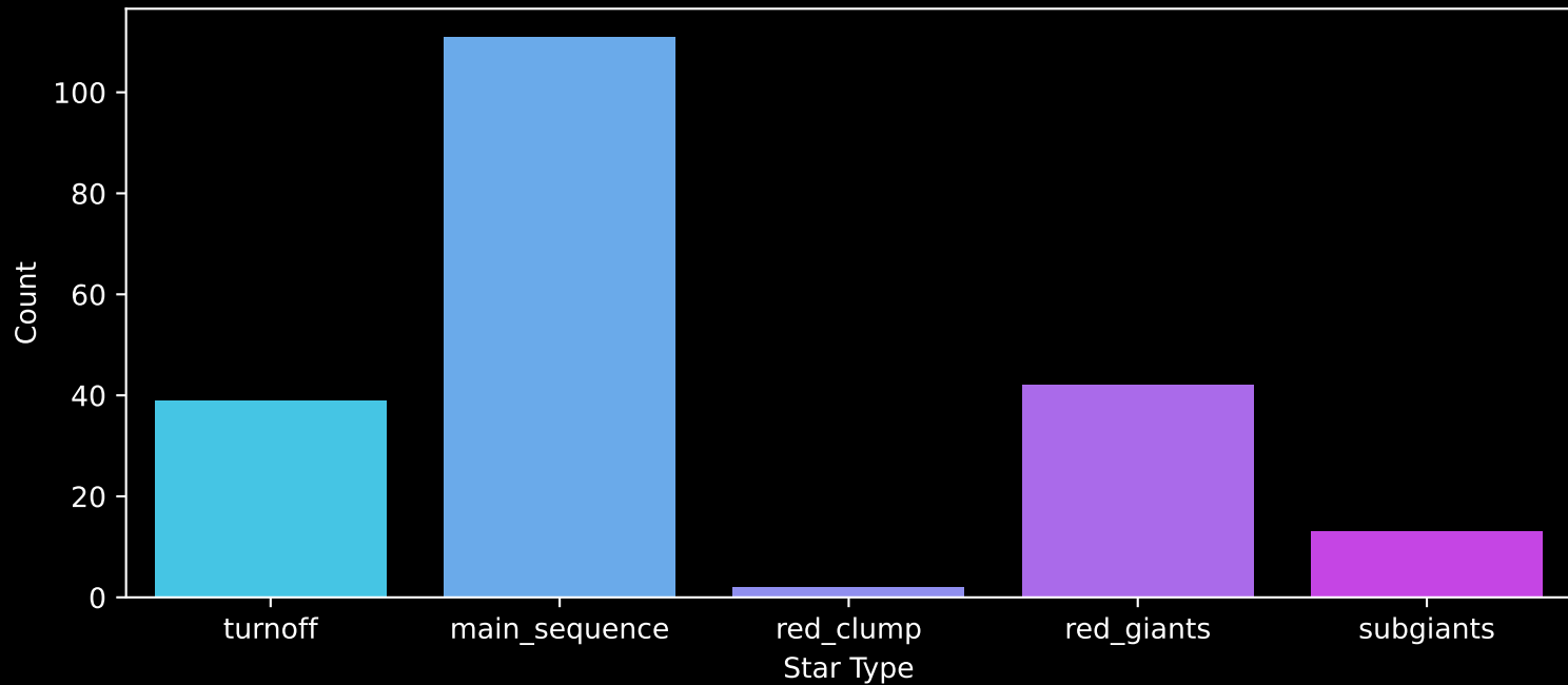
APOGEE DR17 Field: [163+78_MGA] Count plot of Star Type
