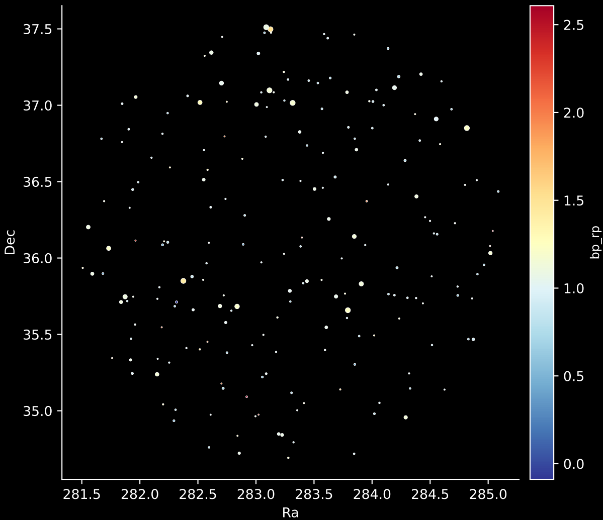
APOGEE DR17 Field: [163+78_MGA] Stars: 207
